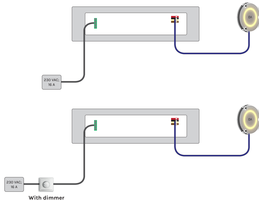
Overview - Combination of MONO SubAqua LED underwater lights and Power Supply Units
