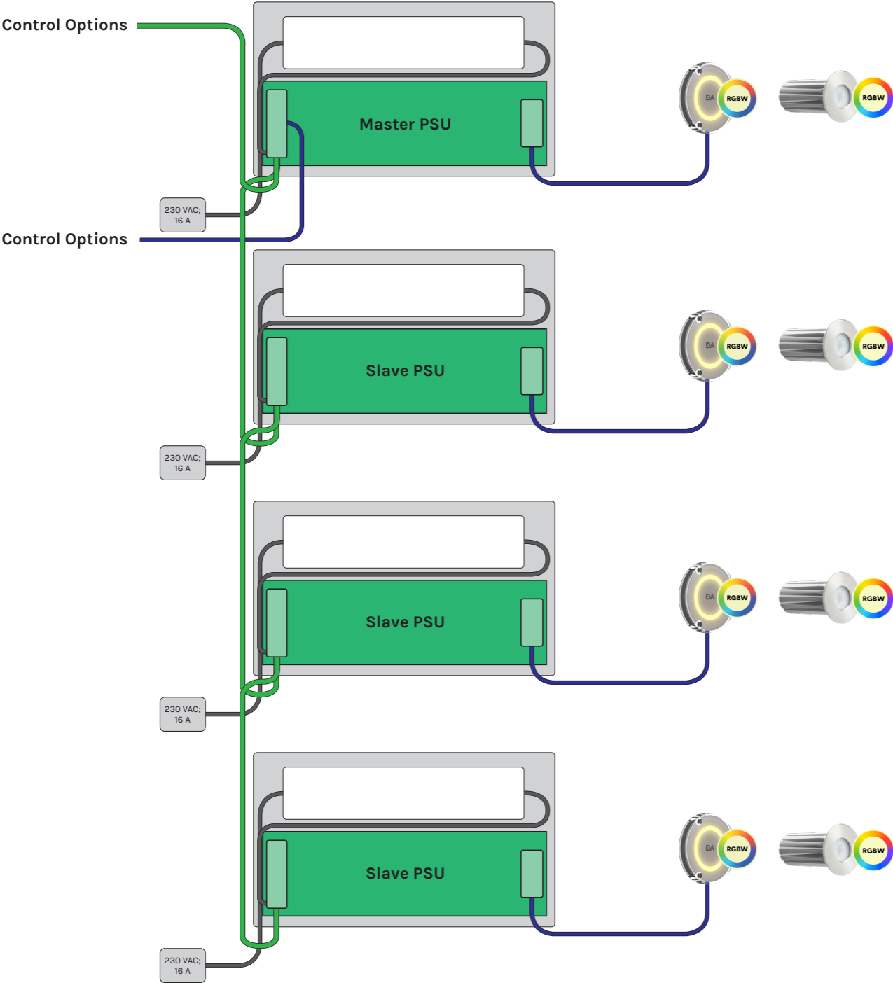
Overview - Combination of RGBW LED underwater lights and Power Supply Units
