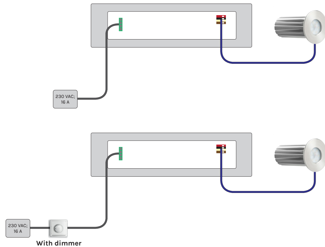
Overview - Combination of B2 underwater lights and Power Supply Units
