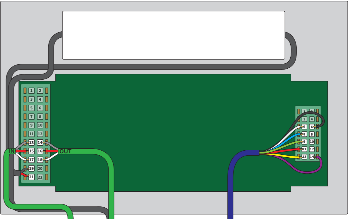
Connections to the Control print of the Power Supply Unit
