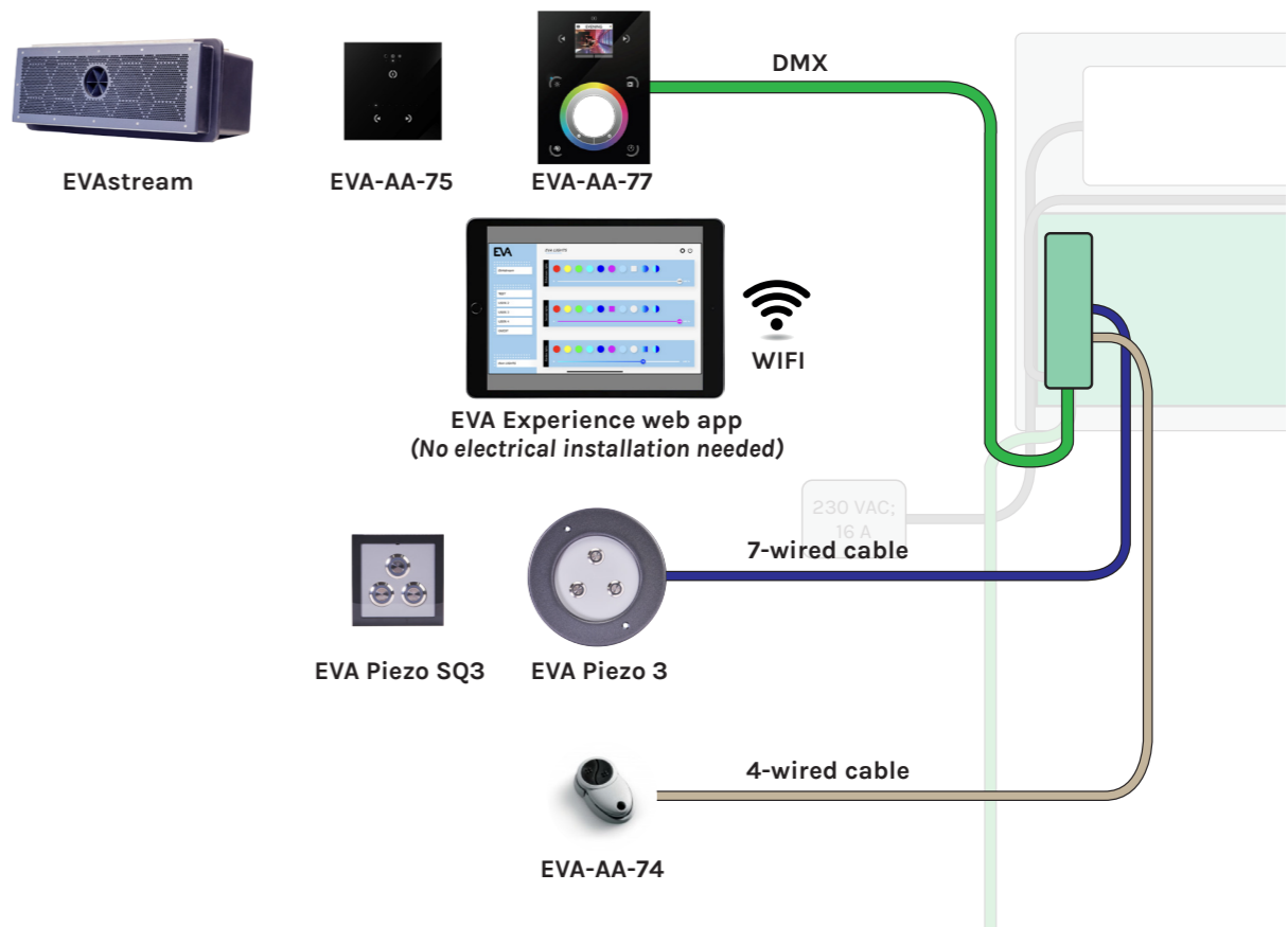
Overview - Control options for RGBW underwater lighting
